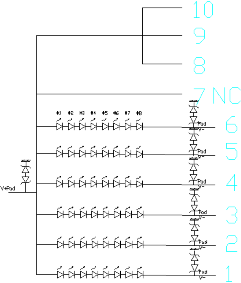
Figure 6. LED Structure
