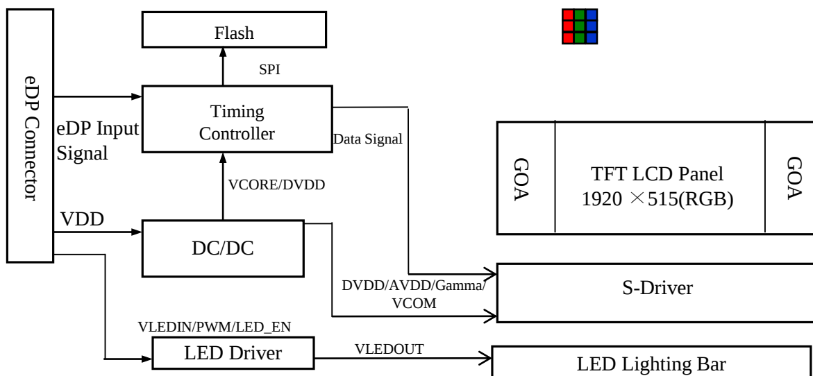
Figure 1. Drive Architecture
