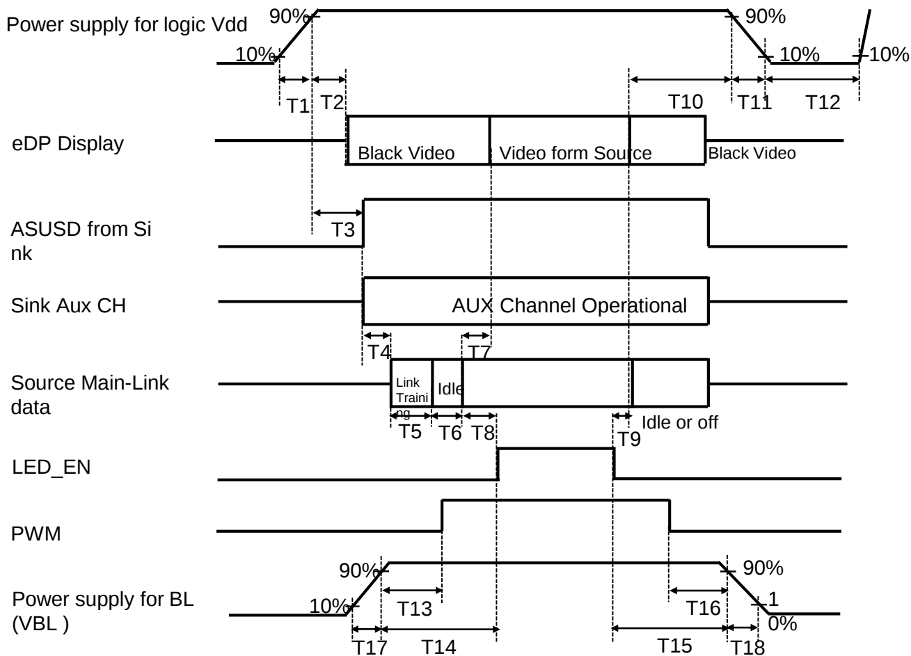
Figure 18. Power Sequence
