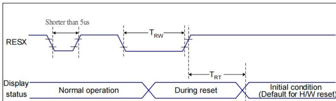
Figure 9 Reset Timing
