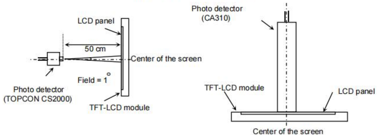
Figure 4. Measurement Set Up
