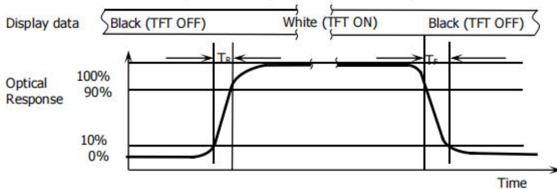
Figure 5. Response Time Testing
