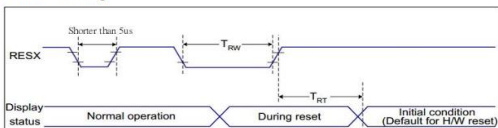
Figure 9 Reset Timing
